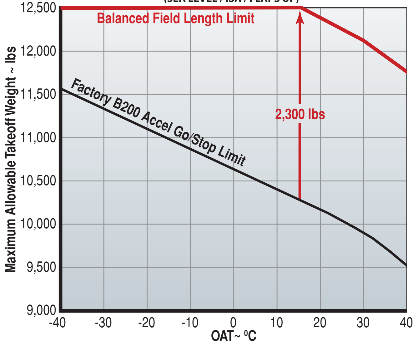
Allowable Takeoff Weight Comparison Raisbeck EPIC B200 vs Factory B200 (SEA LEVEL / ISA / FLAPS UP)
